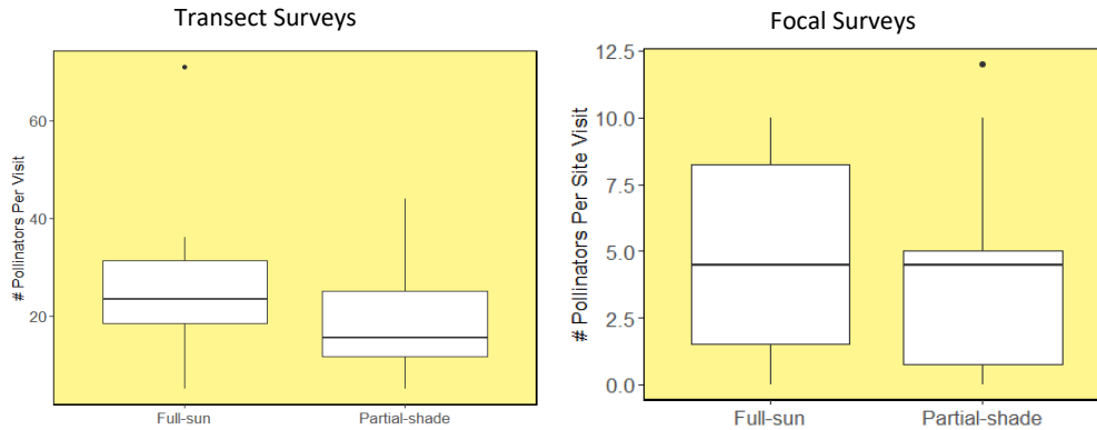
Figure 5. Number of pollinators observed per site visit on transects (left) and focal surveys (right) in full-sun versus partial-shade.
